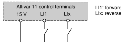
Wiring diagram for 2-wire control
